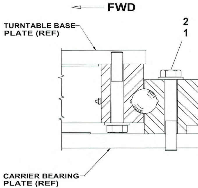
SECTION A-A ROTATED 90° CW
